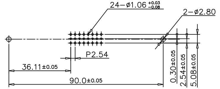
Printed Circuit Board Pattern
